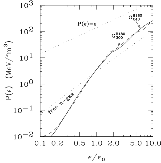
Figure 12.14. Graphical illustration of EOSs G_{B180}^{K240} and G_{B180}^{K300} accounting for quark deconfinement [66]. Details about these EOSs are listed in table 12.4.
