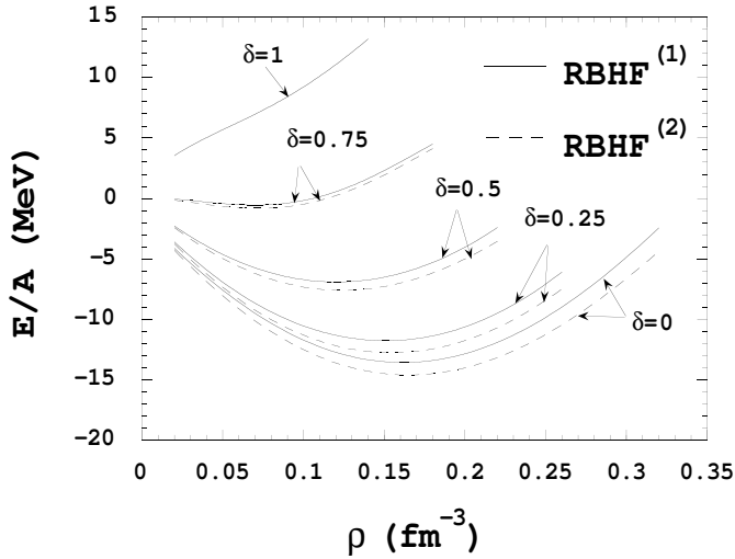
Figure 12.5. Binding energy per nucleon versus density for different asymmetries in the RBHF approximation (BM potential C ) [449]. (Reprinted courtesy of Phys. Rev. )
