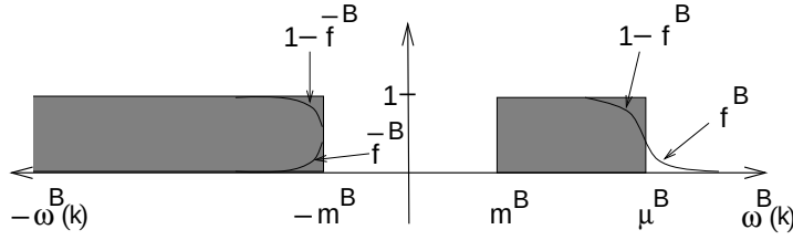
Figure 6.3. Depletion of single-particle states at finite temperature.
