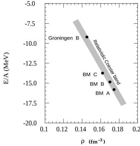
Figure 12.1. Relativistic Coester band associated with \text{RBHF}^{(1)} calculations performed for potentials BM A through BM C, and Groningen B. The data are given in tables 12.1 and 12.2.
