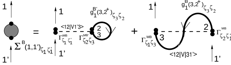
Figure 5.4. Diagrammatic equation of baryon self-energy, \Sigma^B , in Hartree-Fock approximation. The matrix elements \langle 12|\mathbf{V}^{BB'}|1'3 \rangle and \langle 12|\mathbf{V}^{BB'}|31' \rangle , defined in equation (5.151), describe the meson-exchange interaction in the direct (Hartree) and exchange (Fock) term of \Sigma^B , respectively. \Gamma^{MB} and \Gamma^{MB'} denote baryon-meson vertices ( M = \sigma, \omega, \dots ; B = p, n, \Sigma^\pm, \dots ). The analytic expression of \Sigma^B(1, 1') can be inferred from (5.115) in reference to (5.120), or, alternatively, from equations (7.2) and (7.3).
