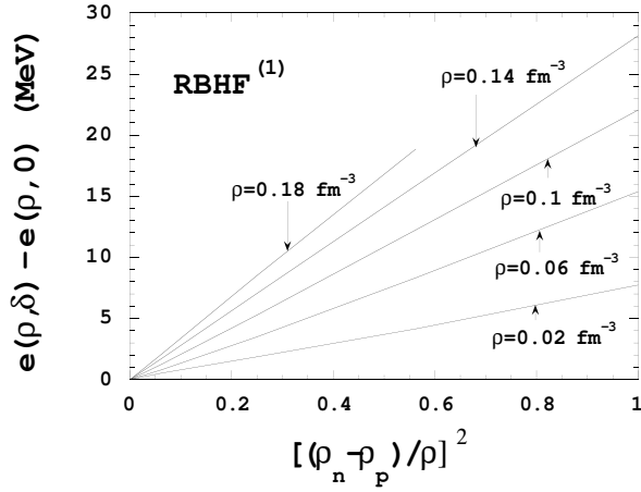
Figure 12.9. Test of the quadratic approximation of the symmetry energy, for five selected densities \rho [449]. The calculations are performed for the RBHF (1) approximation (BM potential A). In accordance with (12.109), the slope of each curve is to a good approximation equal to e^{\text{sym}}(\rho) . (Reprinted courtesy of Phys. Rev. )
