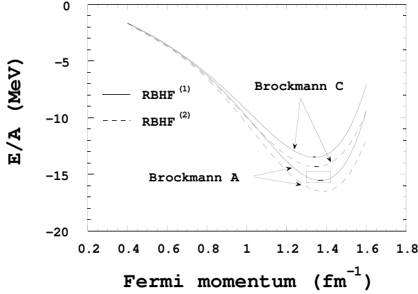
Figure 12.2. Energy per nucleon versus Fermi momentum of symmetric nuclear matter in RBHF for BM potentials A and C [449]. The solid (dashed) curves correspond to the treatment with (averaged) momentum dependency of the self-energies. The square indicates empirical saturation values. (Reprinted courtesy of Phys. Rev. )
