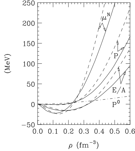
Figure 7.2. Energy per nucleon E/N , chemical nucleon potential \mu^N , and pressure P of cold nuclear matter versus density, for Hartree parameter sets HI (dashed curves) and HII (solid curves) of table 7.2. The dot-dashed curve labeled P^0 shows the pressure of a free relativistic nucleon gas. (Reprinted courtesy of Z. Phys. )
