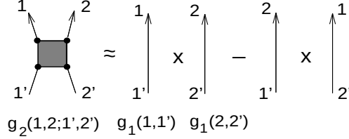
Figure 5.6. Factorization scheme of four-point baryon Green function, g_2 , into antisymmetrized products of two-point baryon Green functions, g_1 \times g_1 [cf. (5.119)]. Direct (Hartree) and exchange (Fock) contribution are shown. This factorization scheme truncates the many-body equations at the Hartree–Fock level.
