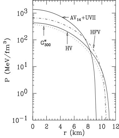
Figure 4.2. Pressure P versus radial distance in non-rotating maximum-mass neutron star models.
