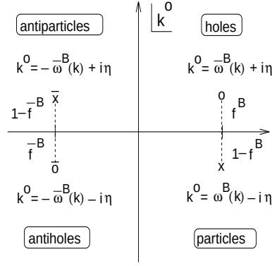
Figure 6.2. Poles of baryon propagator in case of a medium. The crosses ‘x’ and ‘x̄’ refer to the locations of particle and antiparticle poles, respectively. The circles ‘o’ and ‘ō’ denote hole and antihole poles, respectively.
