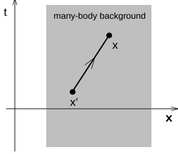
Figure 5.2. Physical interpretation of two-point Green function g_{>}(x, x') defined in equation (5.65): A baryon is created relative to the many-body background (shaded area) at spacetime point x' , propagates to x , where it is removed again.
