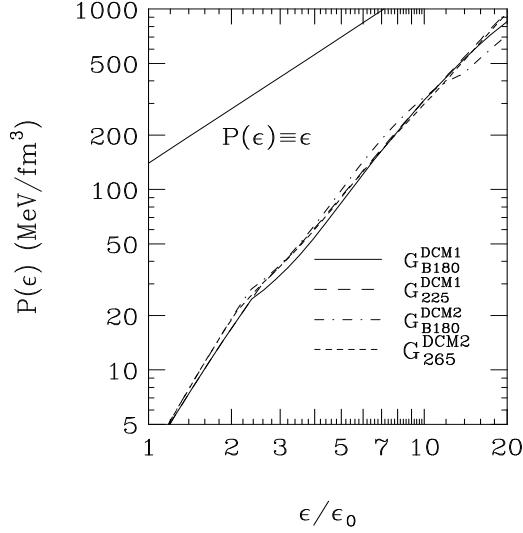
Figure 12.13. Graphical illustration of EOSs G_{B180}^{DCM1} , G_{225}^{DCM1} , G_{B180}^{DCM2} , and G_{265}^{DCM2} [446]. Models G_{B180}^{DCM1} and G_{B180}^{DCM2} account for quark deconfinement. Details about these EOSs are listed in table 12.4.
