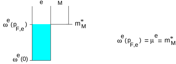
Figure 4.4. Condition for the onset of meson condensation in chemically equilibrated matter. For \mu^e \equiv \omega^e(p_{F,e}) \geq m_M^* high-energy electrons can be replaced with negatively charged mesons ( M = \pi^-, K^- ), which, being bosons, can condense collectively into the ground state.
