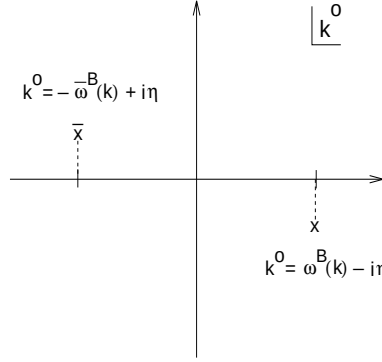
Figure 6.1. Poles of baryon propagator in free space. The symbols ‘x’ and ‘ \bar{x} ’ refer to the locations of particle and antiparticle poles, respectively.
