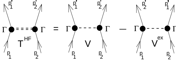
Figure 7.1. Graphical representation of the Hartree–Fock \mathbf{T} -matrix, \mathbf{T}^{\text{HF}} , obtained by restriction to the Born term of the \mathbf{T} -matrix equation (5.203). \Gamma denote baryon–meson vertices listed in (5.156) through (5.158). The analytic form of \mathbf{T}^{\text{HF}} is given in equation (7.1).
