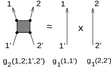
Figure 5.7. Factorization scheme of four-point baryon Green function, g_2 , into a product of two-point baryon Green functions, g_1 \times g_1 . Keeping only the first term of (5.119), this truncates the many-body equations at the Hartree level.
