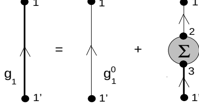
Figure 5.3. Graphical representation of Dyson's equation for the self-consistent two-point baryon Green function g_1 . The quantity g_1^0 denotes the propagator of free baryons, which do not feel the nuclear medium (i.e. \Sigma \equiv 0 ). The momentum-space representation of Dyson's equation is given in (5.126).
