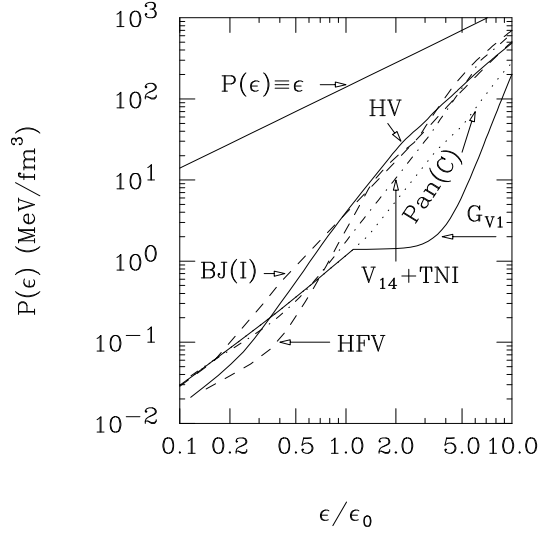
Figure 12.10. Graphical illustration of EOSs BJ(I), Pan(C), V_{14} + \text{TNI} , HV, and HFV [446]. Details about these EOSs are listed in table 12.4.
