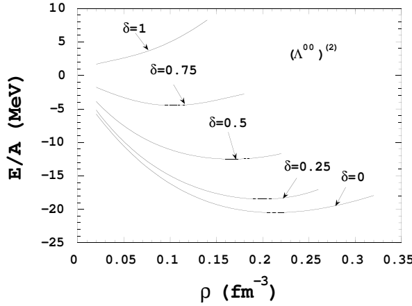
Figure 12.6. Binding energy per nucleon versus density for different asymmetries in the \Lambda^{00} approximation (BM potential C ) [449]. (Reprinted courtesy of Phys. Rev. )
