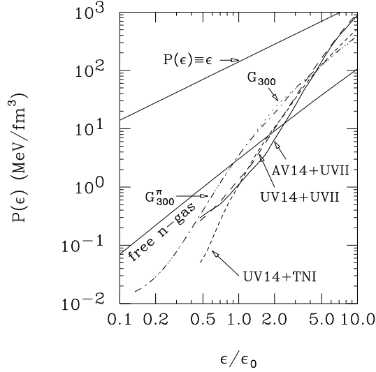
Figure 12.11. Graphical illustration of EOSs AV_{14} + UV_{II} , UV_{14} + UV_{II} , UV_{14}+TNI , G_{300} , and G_{300}^{\pi} [446]. Details about these EOSs are listed in table 12.4.
