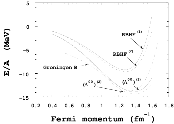
Figure 12.3. Energy per nucleon of nuclear matter computed for different many-body approximations [449]. The underlying potential in each case is Groningen B. The individual approximations are, \text{RBHF}^{(1)} and \Lambda^{00(1)} : relativistic \mathbf{T} -matrix calculation in RBHF and \Lambda^{00} approximation where full momentum dependence of self-energy is kept; \text{RBHF}^{(2)} and \Lambda^{00(2)} : same as \text{RBHF}^{(1)} and \Lambda^{00(1)} but for momentum averaged self-energy; Groningen B: RBHF calculation based on the decomposition of the \mathbf{T} -matrix into the Fermi invariants listed in equation (12.108). (Reprinted courtesy of Phys. Rev. )
