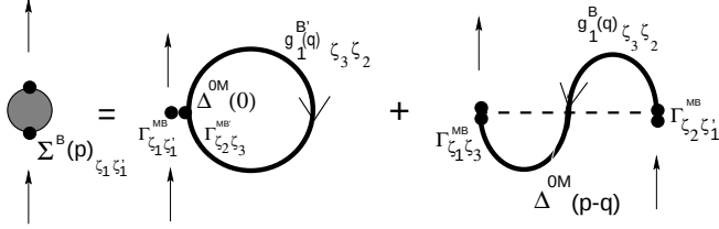
Figure 5.5. Diagrammatic representation of Hartree-Fock baryon self-energy \Sigma^B in momentum space. \Delta^{0M}(0) and \Delta^{0M}(p - q) denote meson propagators, derived, for instance, in equations (5.93) and (5.100). All other quantities are explained in figure 5.4. For the analytic form of \Sigma^B(p) , see, for example, equations (5.134) through (5.142).
