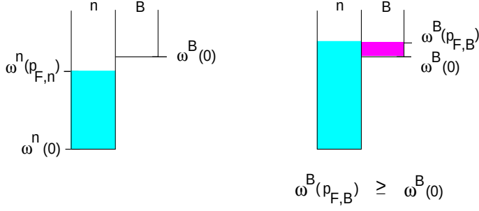
Figure 4.3. Condition for the onset of hyperon population in chemically equilibrated matter. Left: the single-particle energy is not high enough for the neutrons to transform to baryons of type B . Right: high-energy neutrons overcome the baryon threshold, that is, \mu^B \equiv \omega^B(p_{FB}) \geq \omega^B(0) , and therefore transform to particle state B .
