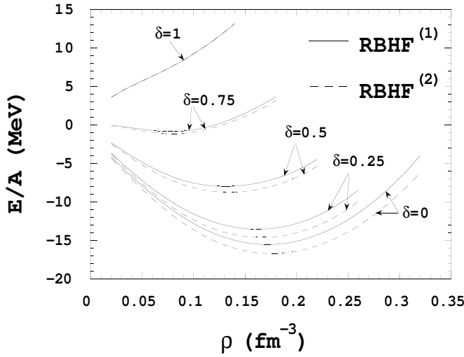
Figure 12.4. Binding energy per nucleon versus density for different asymmetries in the RBHF approximation (BM potential A) [449]. (Reprinted courtesy of Phys. Rev. )
