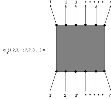
Figure 5.1. Graphical representation of the 2n -point Green function defined in equation (5.62). The vertical lines denote the propagation of baryons in and out of the many-body vertex (shaded area).
