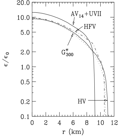
Figure 4.1. Energy density \epsilon (in units of normal nuclear matter density, \epsilon_0 ) versus radial distance in non-rotating maximum-mass neutron star models.
