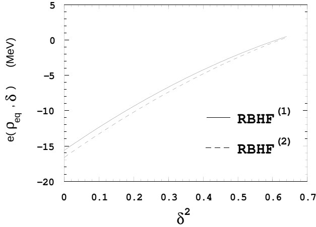
Figure 12.7. Energy per particle (11.4) at equilibrium as a function of asymmetry \delta , computed for BM potential A [449]. (Reprinted courtesy of Phys. Rev. )
