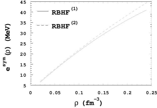
Figure 12.8. Symmetry energy (11.5) as a function of density computed for BM potential A [449]. (Reprinted courtesy of Phys. Rev. )
