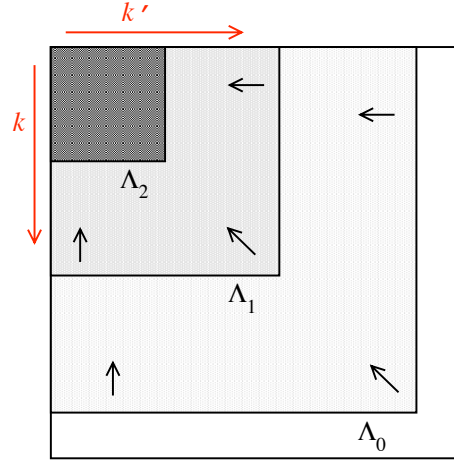
Figure 1.9: Evolution of the matrix elements of the V_s = V_{low-k} as a function of the sharp cutoff \Lambda .
