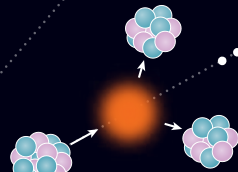
Nuclear fission
