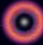
Supernovae
