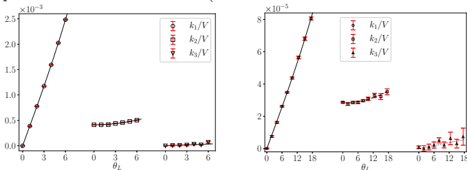
Imaginary- \theta fit. Left: 2d CP^{N-1} models. Right: 4d SU(N) pure-gauge theories.
