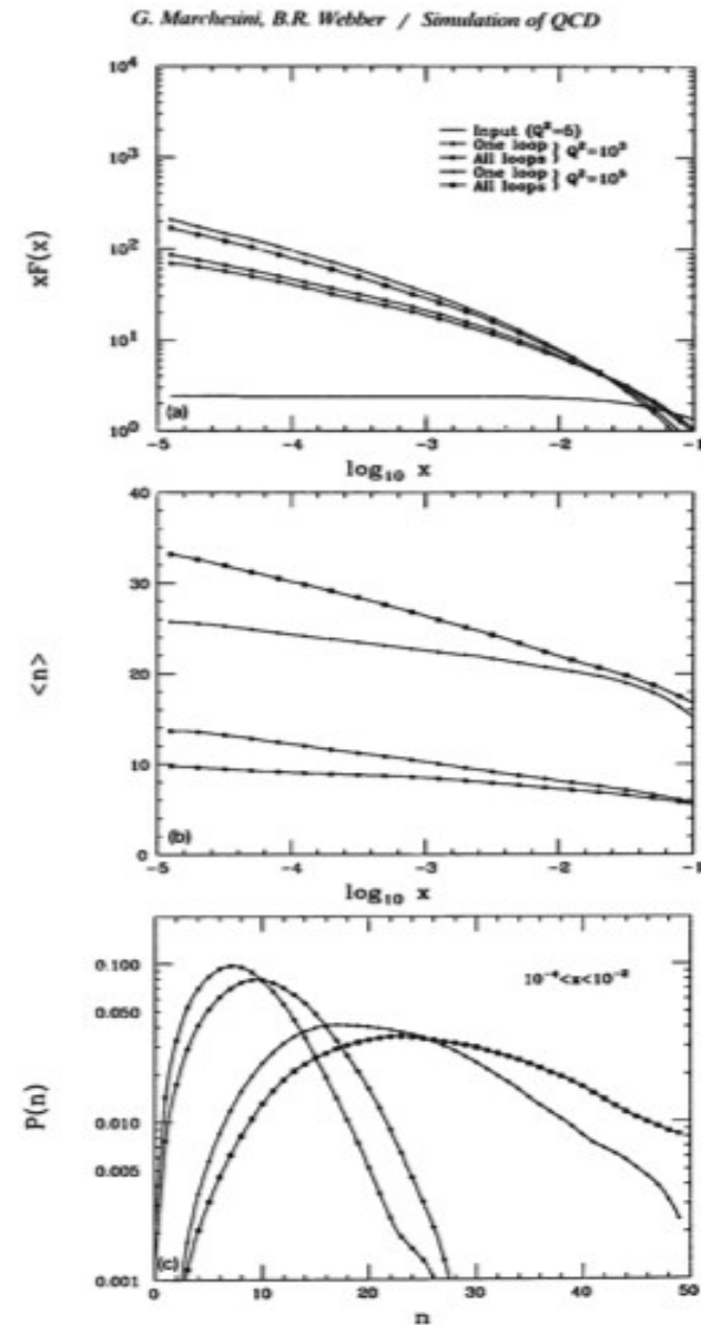
Fig. 2. Results for flat input structure function, xF(x, Q_0) = A(1-x)^5 .
